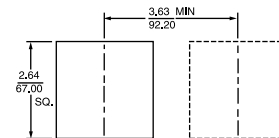
PANEL CUTOUT SHOWING DISTANCE BETWEEN ADJACENT CUTOUTS.
