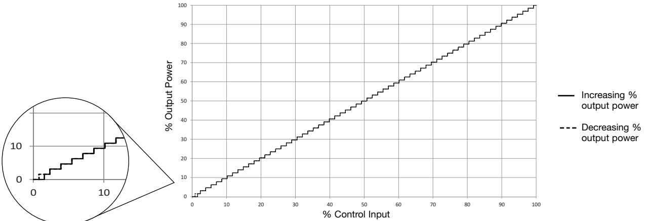
1 Full cycle switching mode: RGC...C1
