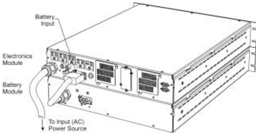
Figure 3 Power Connections
