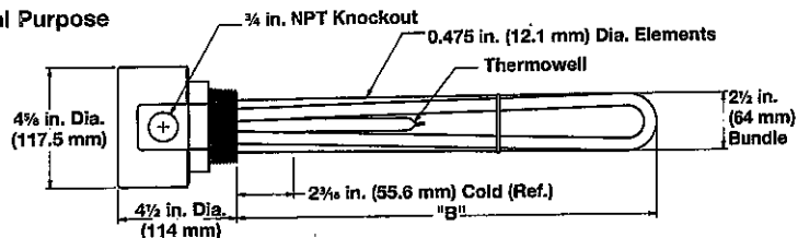
Moisture/Explosion-Resistant
