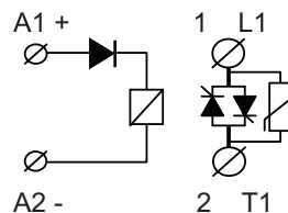
DC Controlled
