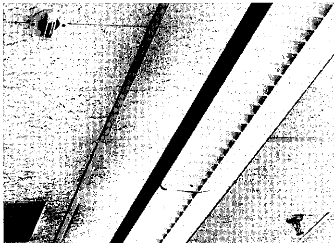
Figure 5. Typical ceiling installation of a horizontal DETECT-A-FIRE model. Here it is used in combination with a sprinkler system to detect overheat and actuate an alarm.
