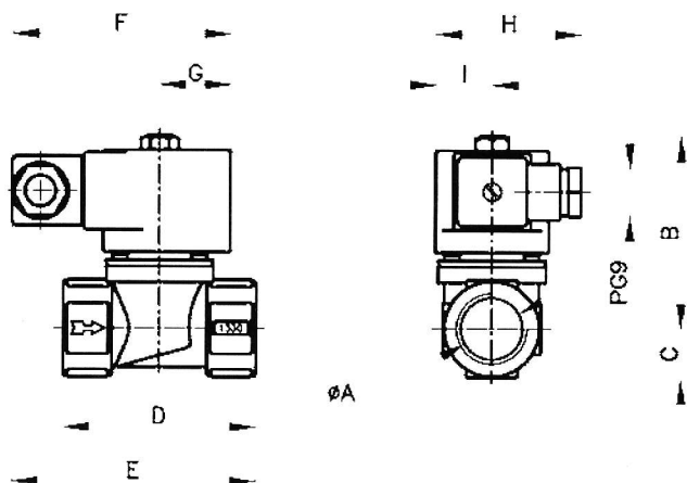
DIRECT ACTING
