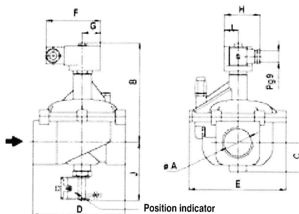
PILOT OPERATED
